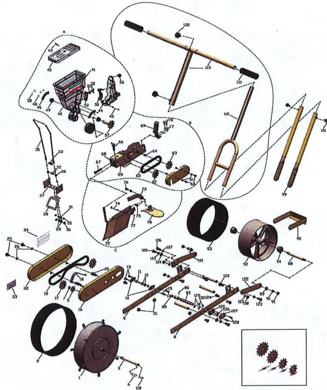
Sprocket Gear (9,10,13,14T)
