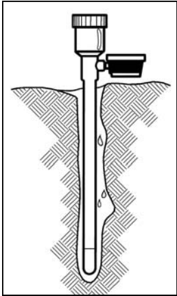
Poor Installation
